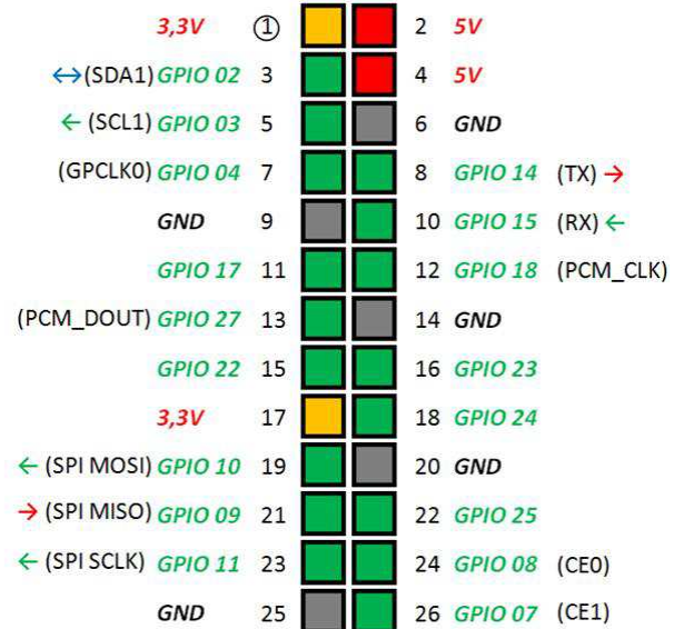
Raspberry Pi Rev 2
