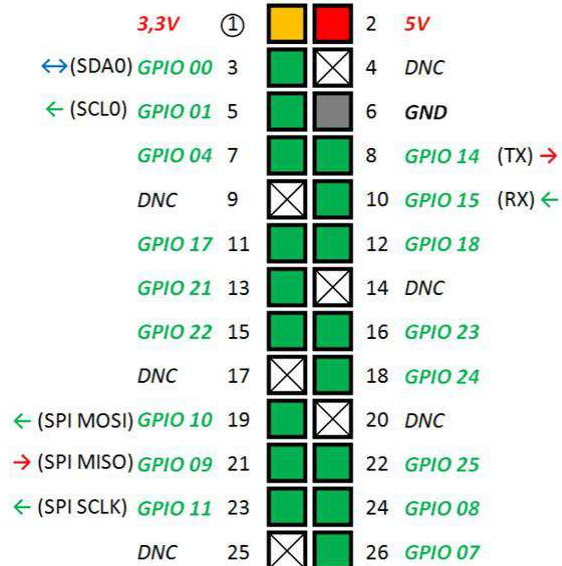
Raspberry Pi Rev 1
